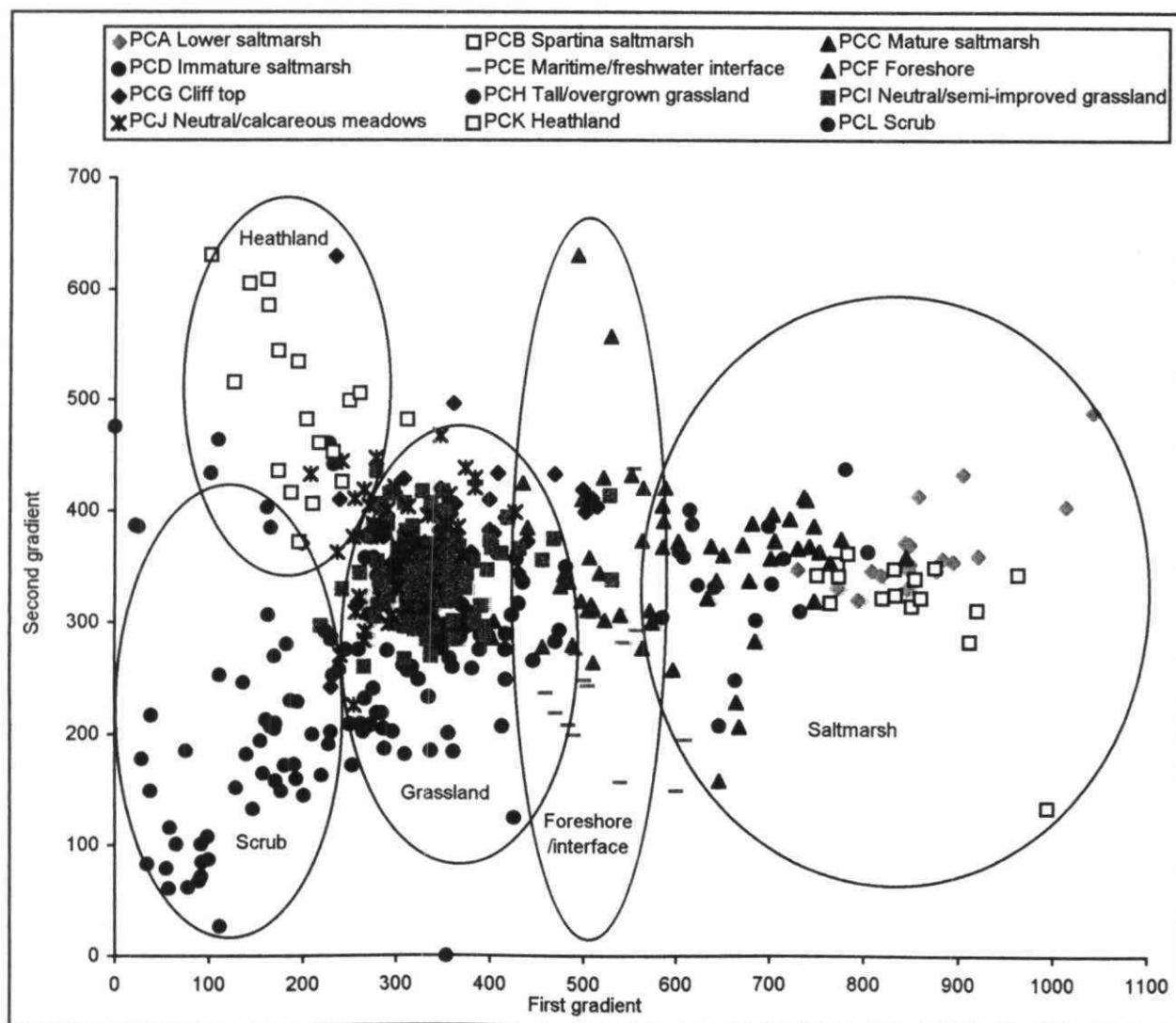
Figure 4.4 Coastal quadrats - ordination diagram using DECORANA scores
