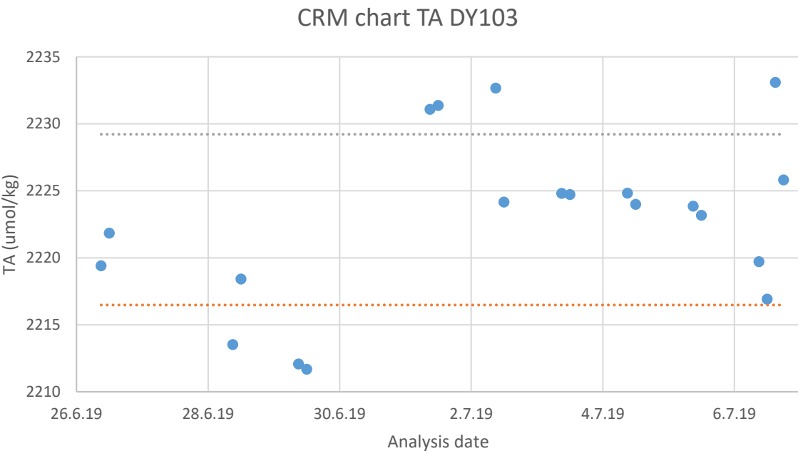
Range charts for Vindta CRM showing \pm 1sd of the cruise average for a) DIC and b) TA
