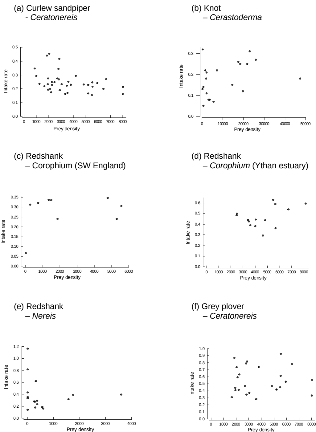
Figure 3.1 Functional responses of waders eating macro-invertebrates: intake rate (mg AFDM s^{-1} ) against numerical density of the prey (number m^{-2} ). In oystercatchers eating mussels or cockles, the method of feeding is given; stabbing between the shell valves or hammering into shells on the dorsal or ventral sides. Species are shown in ascending order of body size.
