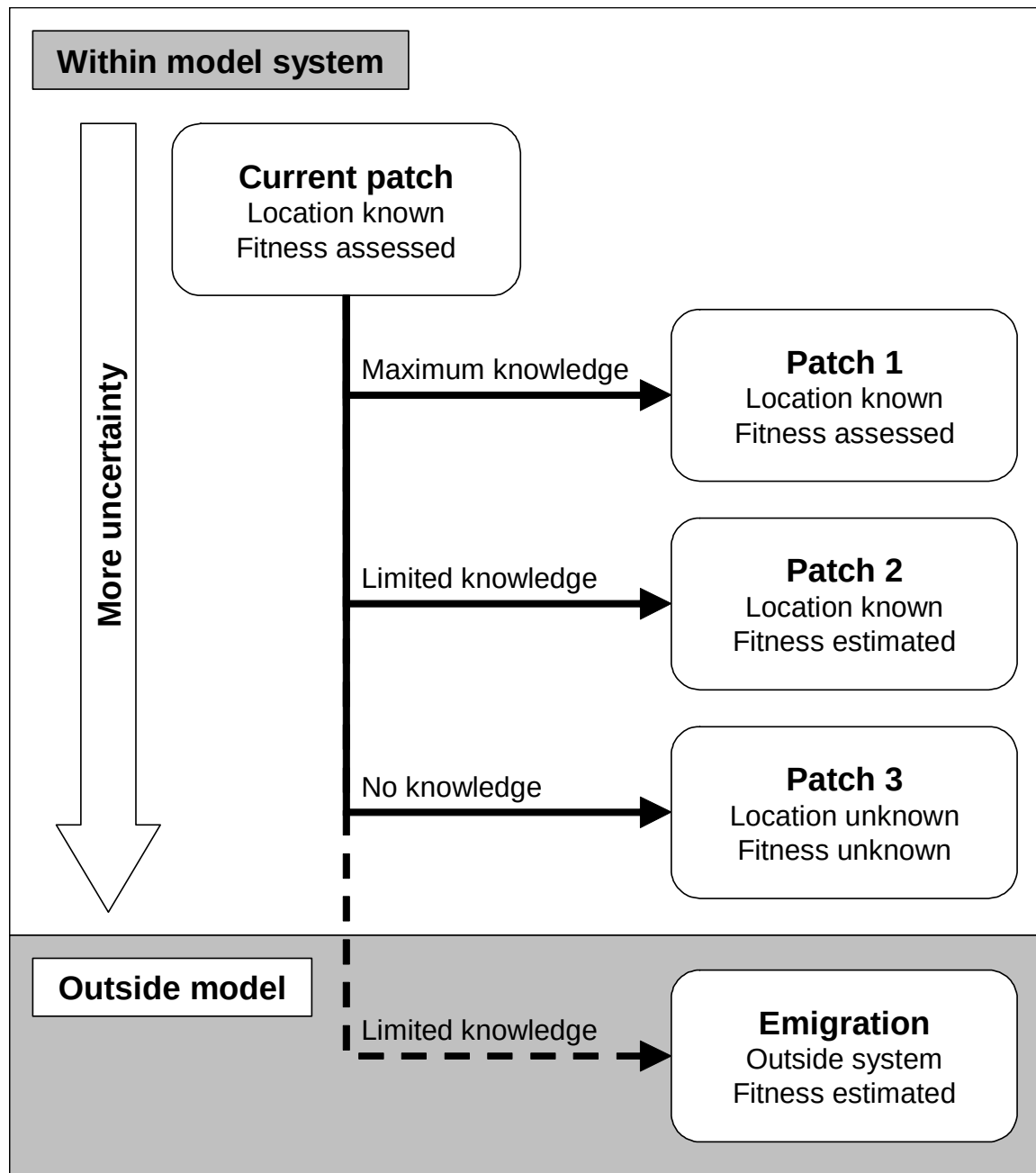
Figure 2.2 How uncertainty is incorporated into the model. Foragers are assumed to be able to assess the fitness measure associated with consuming different diets on their current patch. Other patches fall into one of three different categories. (1) Foragers may know the location of a different patch and be able to assess fitness measures on the patch (e.g. Patch 1). (2) Foragers may know the location of a patch, but not be able to assess the fitness measures associated with different diets (e.g. Patch 2). In this case the estimated fitness measure on the patch is used. (3) Patches may be of unknown location (e.g. Patch 3). Emigration from the system also has an expected fitness measure. Although, the figure shows increasing uncertainty associated with increasing distance between patches, this does not have to be the case.
